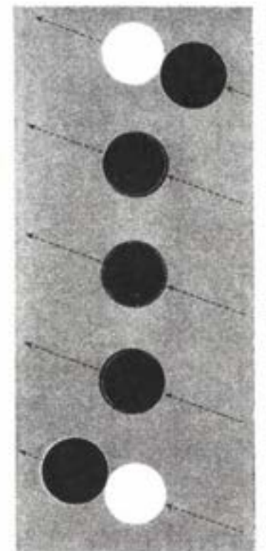
Fig. 322 Total eclipse
